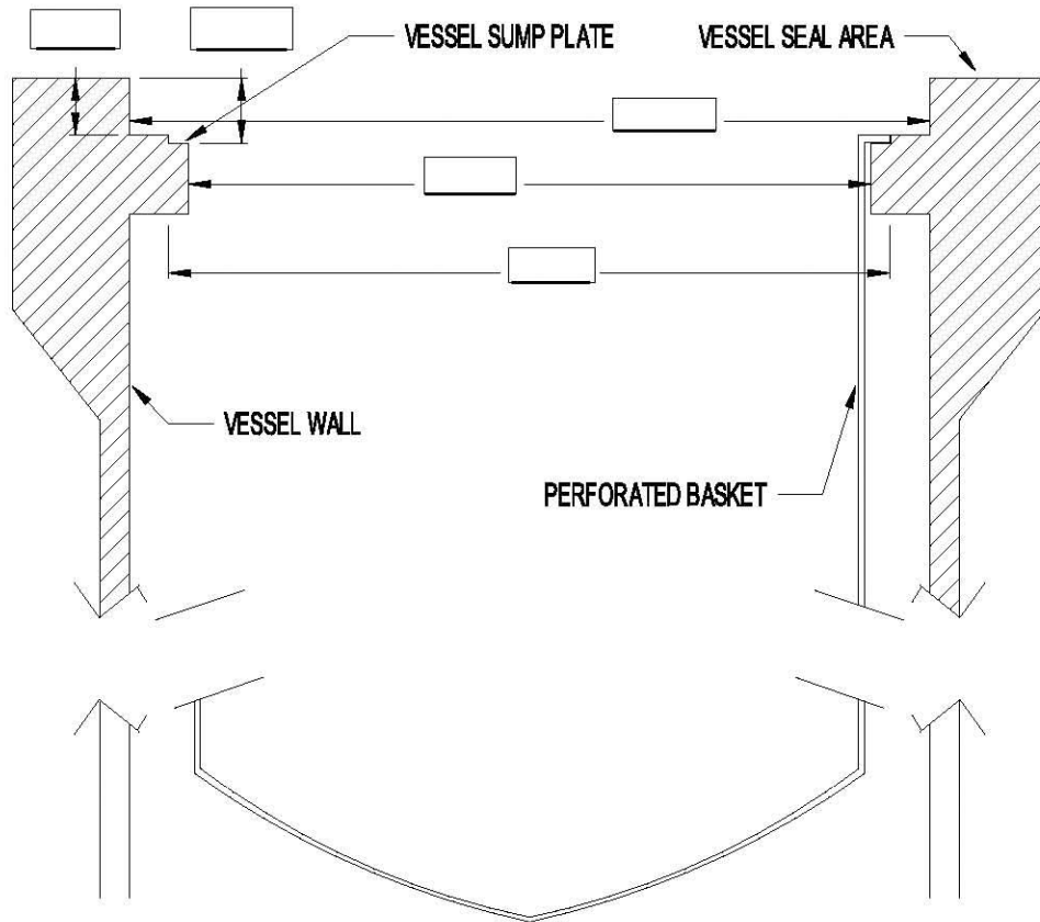
VESSEL - SECTION VIEW
