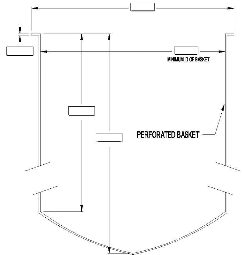
BASKET - SECTION VIEW
