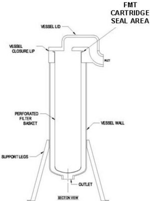
TYPICAL SINGLE BAG HOUSING
