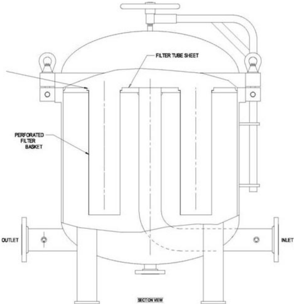
TYPICAL MULTI-BAG HOUSING
